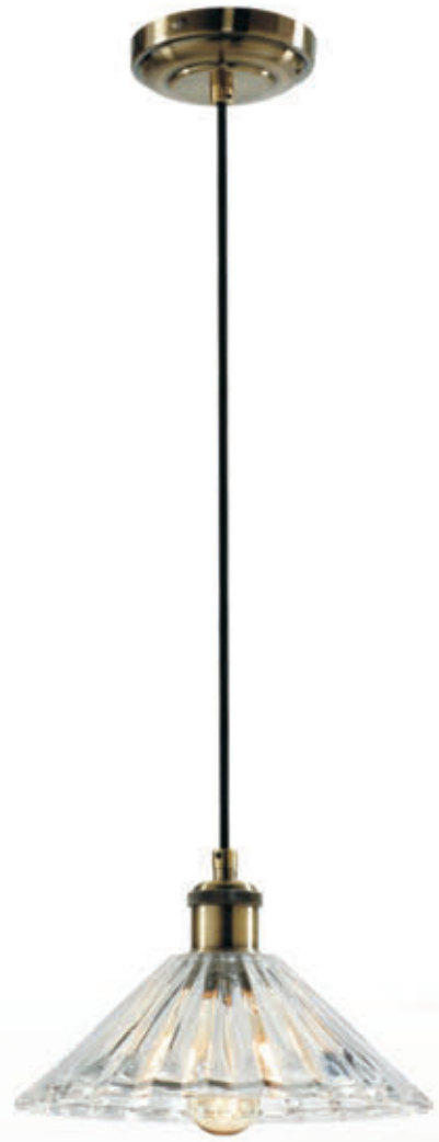
PEN88408 antique brass/clear metal/glass Max. 60W E27x1 Ø245xH1200mm
