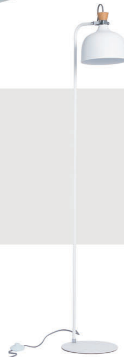
F88418WH-A white metal/wood Max. 60W E27x1 390x300xH1460mm
